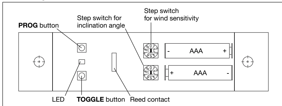
Picture 1: Housing cover – view inside on the board
